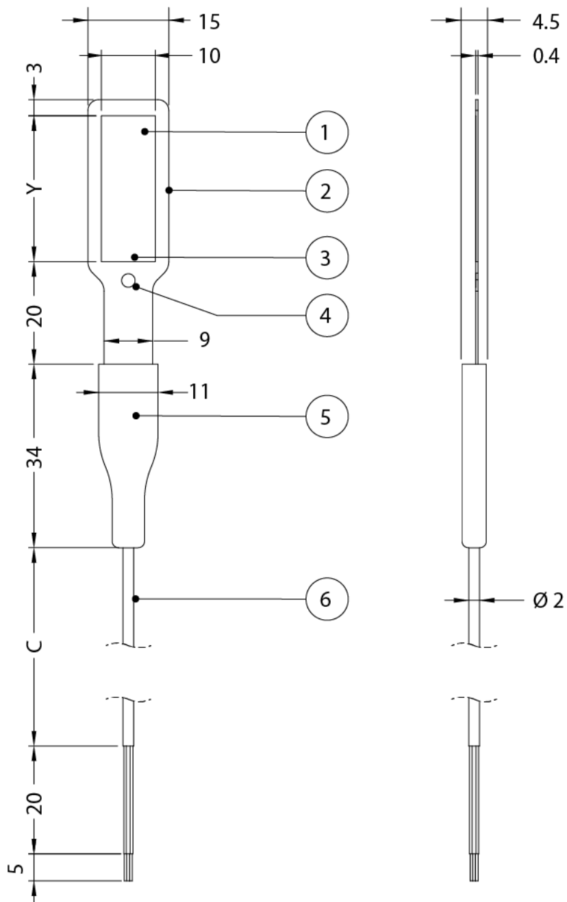
Figure 3.2.1 Models FHF05 15X30 and 15X85; Y_1 = 27 or 70 , Y_2 = 18 or 25 with dimensions in \times 10^{-3} m
