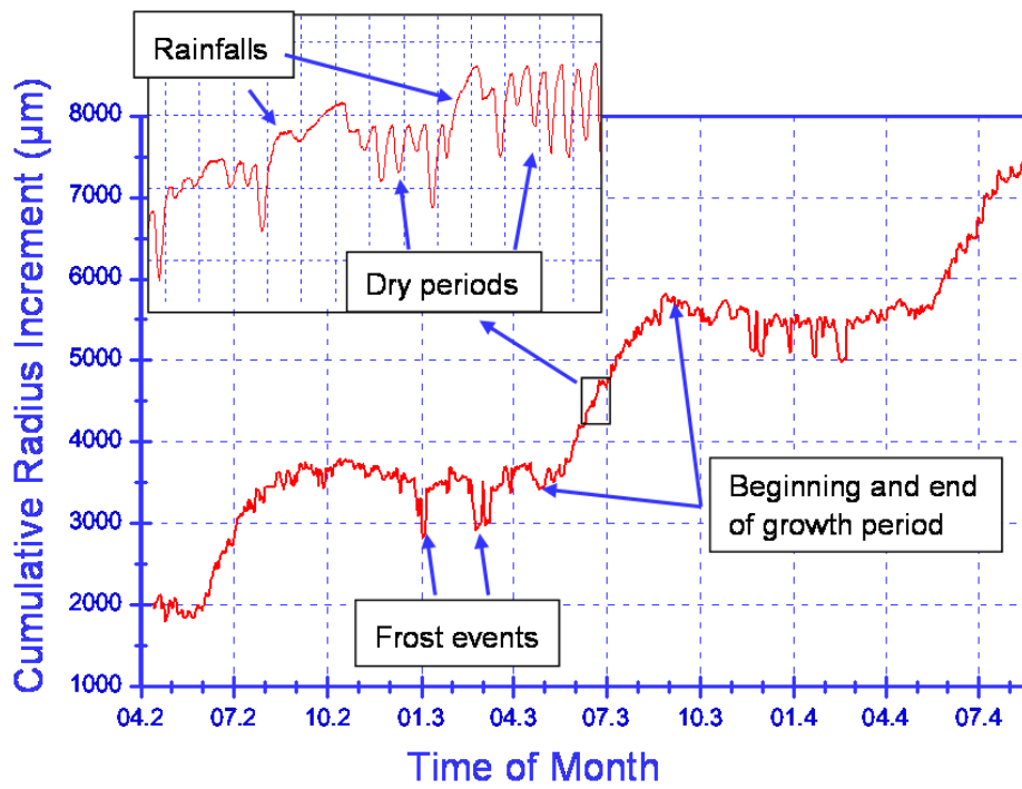
Fig. 1 Growth curve of a spruce tree
